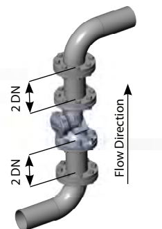
2 pipe diameters before and after elbows (90°) in vertical installations
