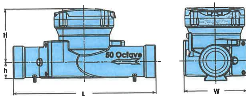
Picture No.8 Installation dimensions - Threaded
