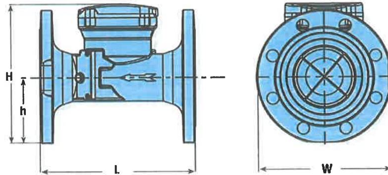
Picture No.9 Installation dimensions - Flanged
